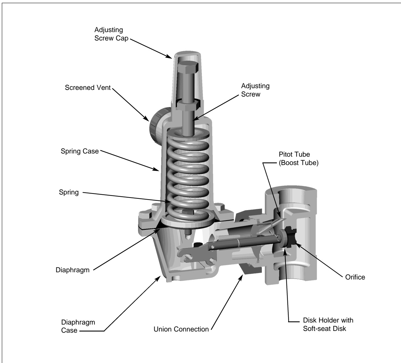
Figure 2. Model 5646 Cross-sectional View
